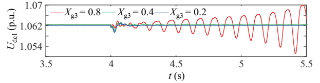
Fig. 11. Time domain responses of DC voltage of VSC 1 with different transmission line reactance of VSC 3.
