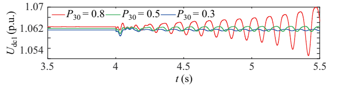
Fig. 12. Time domain responses of DC voltage of VSC 1 with different active power of VSC 3.
